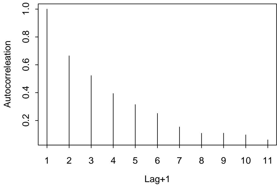
Empirical ACF for Simulated AR(1)
