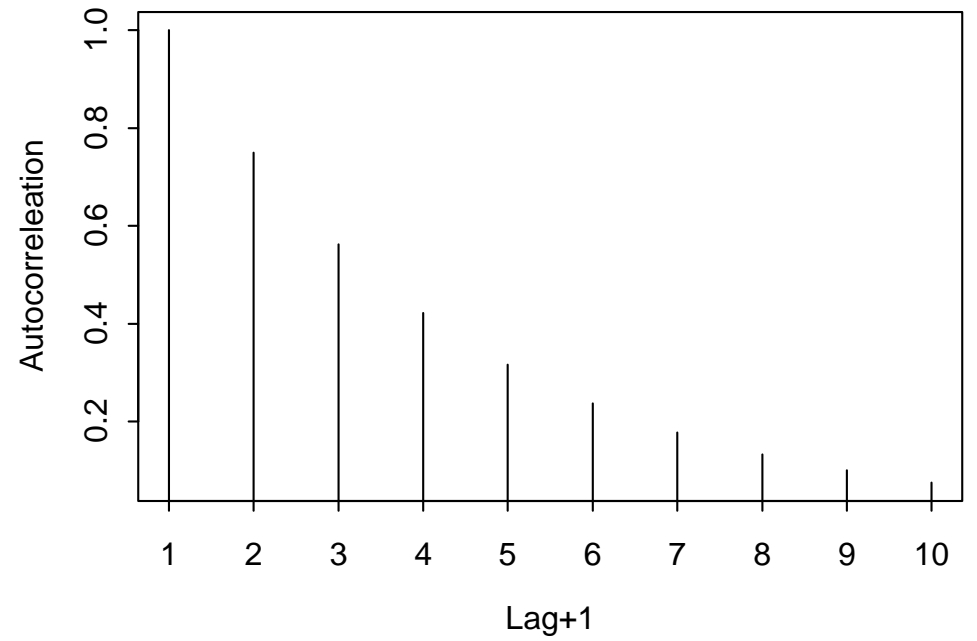
Theoretical ACF for AR(1)
