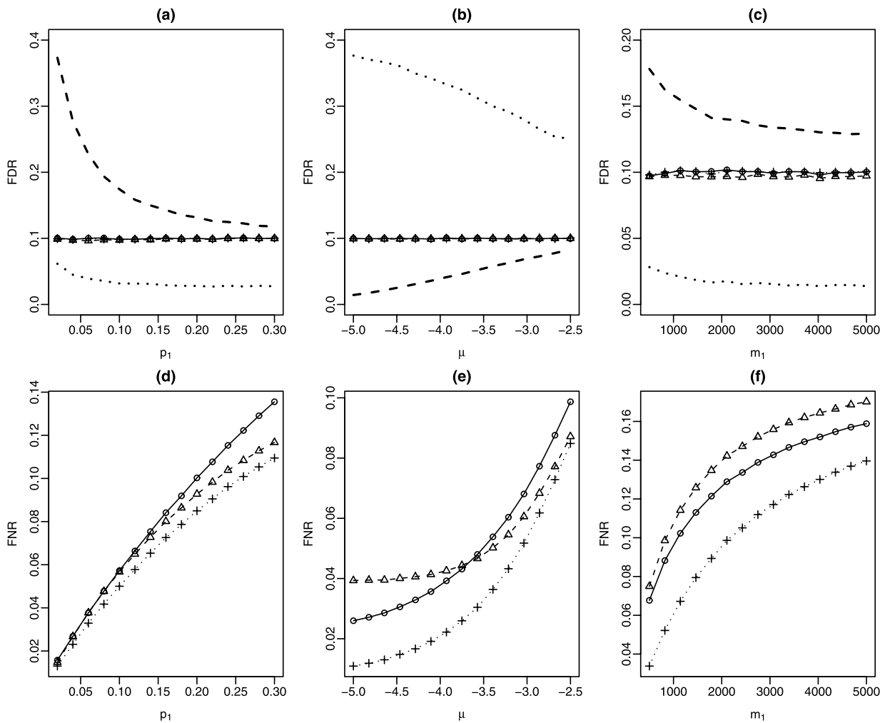
Figure 4. Results for Simulation study 1: the top row compares the FDR levels and the bottom row compares the FNR levels (○, PLfdr; △, SLfdr; +, CLfdr). The optimal group-wise FDR levels suggested by the CLfdr procedure are provided together with the global FDR levels (dashed line, group 1; dotted line, group 2).
