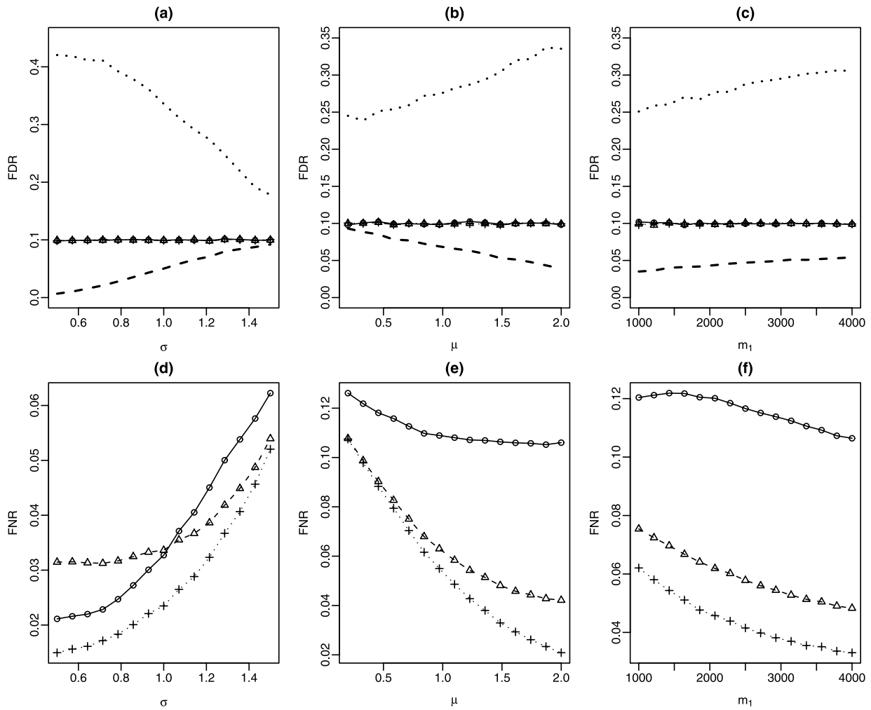
Figure 5. Results for Simulation study 2: the top row compares the FDR levels and the bottom row compares the FNR levels (○, PLfdr; △, SLfdr; +, CLfdr). The optimal group-wise FDR levels suggested by the CLfdr procedure are provided together with the global FDR levels (dashed line, group 1; dotted line, group 2).
