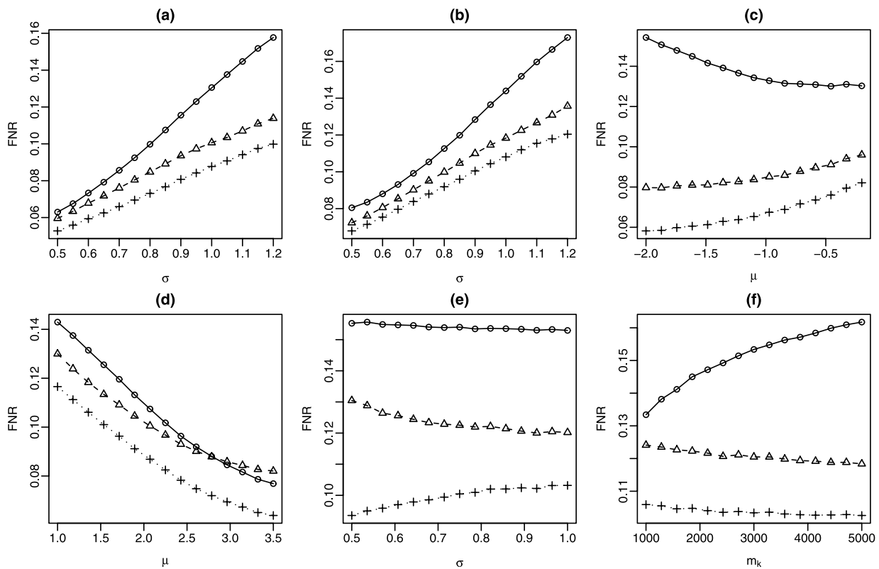
Figure 6. Results for Simulation study 3. The FNR levels of PLfdr, SLfdr, and CLfdr procedures are plotted as functions of model parameters (○, PLfdr; △, SLfdr; +, CLfdr). The first row compares oracle procedures and the second row compares data-driven procedures. Detailed simulation settings are summarized in Table 2.
