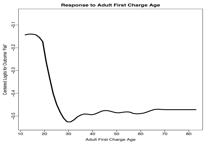
Figure 6: Random Forests Partial Dependence Plot for “Adult First Charge Age”
