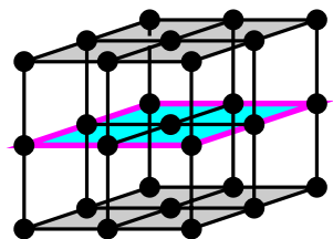
Fig. 1.1. The discrete Loomis-Whitney inequality tells that for any collection A of points in \mathbb{R}^3 one has |A| \leq |A_x|^{\frac{1}{2}} |A_y|^{\frac{1}{2}} |A_z|^{\frac{1}{2}} . The cubic arrangement indicated here suggests the canonical situation where one finds the case of equality in the bound.
