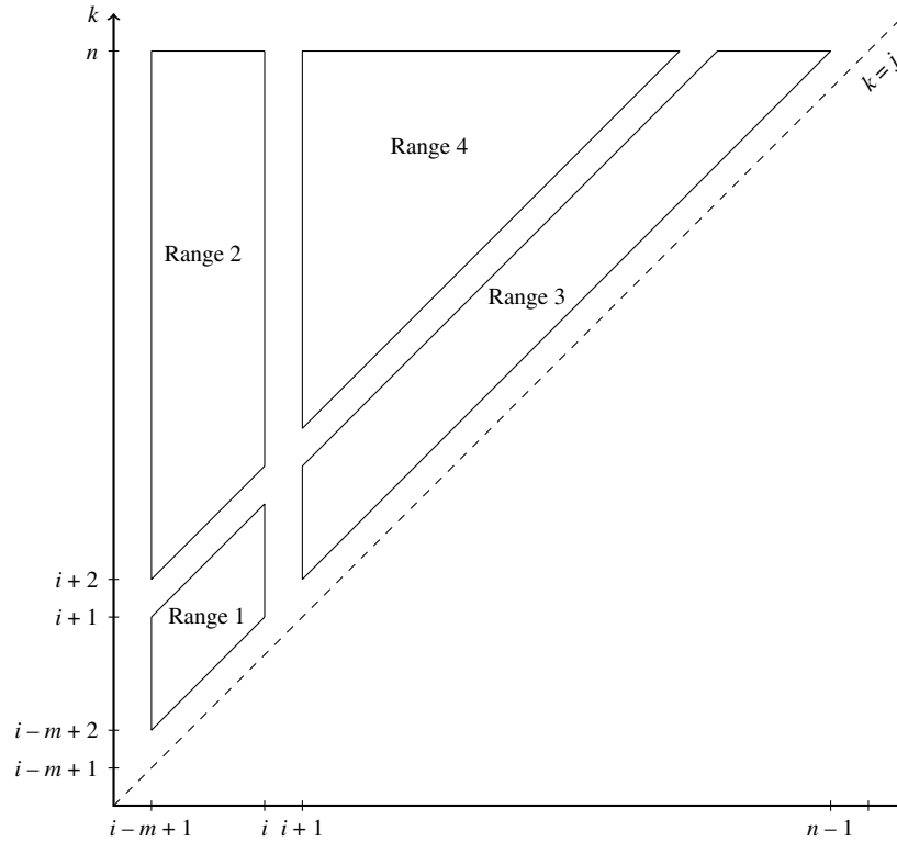
FIGURE 1. Cross moments index relations.
