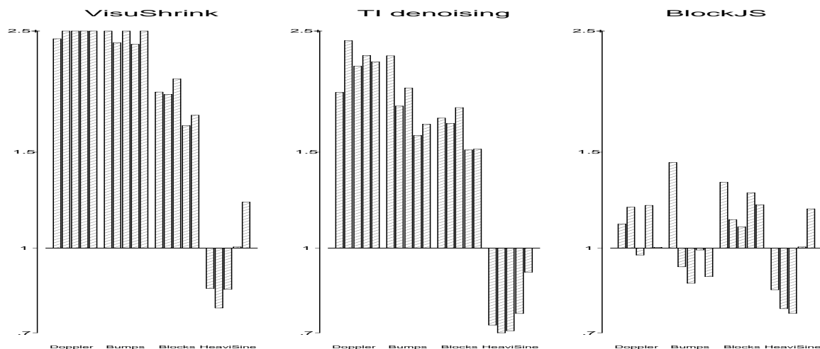
Figure 1: Comparison of MSEs. For each signal the bars are ordered from left to right by the sample sizes ( n=512 to 8192 ). The higher the bar the better the relative performance of \tilde{f}^* .
